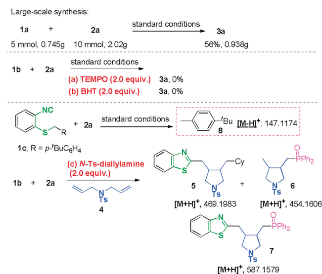
Scheme 4. Large-scale synthesis and radical inhibiting experiments.
