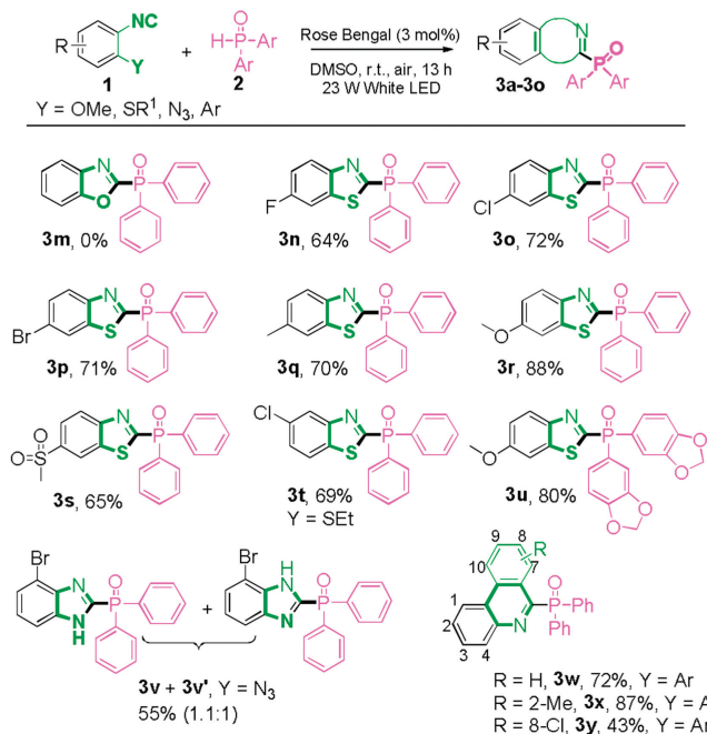
Scheme 3. Substrates scope on isocyanides. Reaction conditions: Isocyanides ( 1 , 0.15 mmol), H -phosphorus oxides ( 2 , 0.3 mmol), Rose Bengal (3 mol%), 1.5 mL of DMSO, 23 W white LED for 13 h under air, isolated yields, Y = SMe (unless stated).
