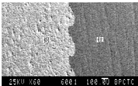
图2 钛/钢爆炸焊接界面的扫描电镜显微照片 Fig. 2 Micrograph of titanium-steel explosive welding interface by scanning electron microscope
