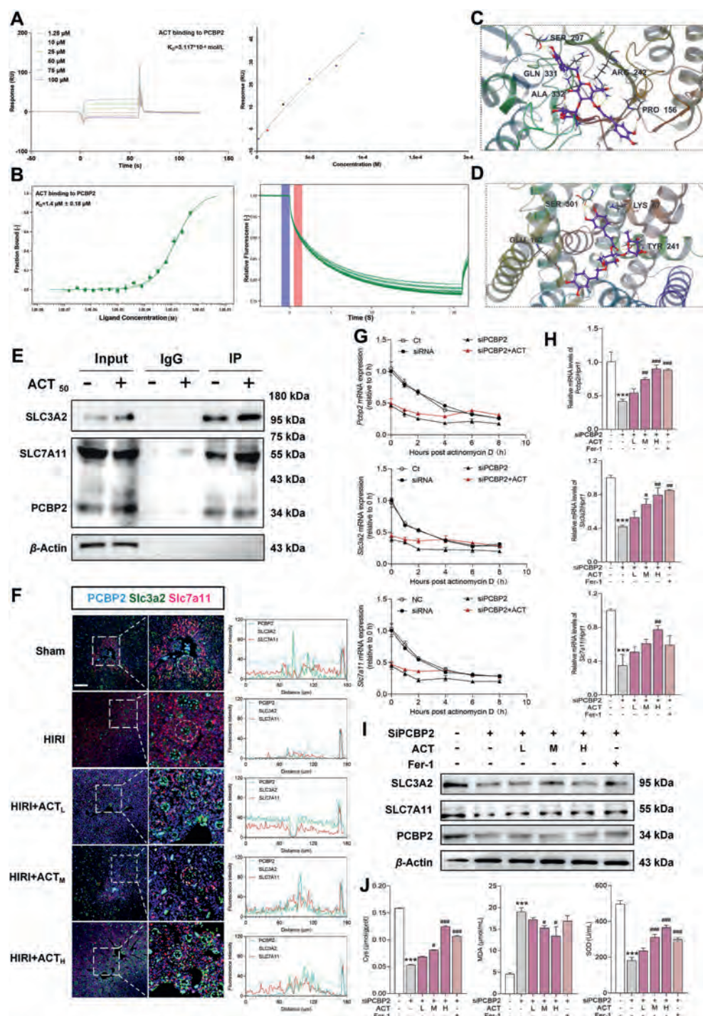
Figure 5 ACT promotes PCBP2 to maintain the stability of system Xc - . (A) The SPR detection of ACT with PCBP2 protein. (B) The MST results of ACT with PCBP2 protein. (C) The molecular simulation docking between ACT and PCBP2–SLC3A2 protein complex. (D) The molecular simulation docking between ACT and PCBP2–SLC7A11 protein complex. (E) The co-IP results between PCBP2 and SLC3A2/SLC7A11. (F) The representative images of multi-color fluorescence staining of PCBP2/SLC3A2/SLC7A11 in mouse livers, scale bar = 40 μm. (G) The mRNA changes of Pcbp2 , Slc3a2 and Slc7a11 in hepatocytes. (H) Relative mRNA levels of Slc3a2 , Slc7a11 and Pcbp2 in AML12 cells were measured by qPCR and further normalized with hprt1 . Statistical significance: *** P < 0.001, compared with control group; # P < 0.05, ## P < 0.01, ### P < 0.001, compared with the siPCBP2 group ( n = 3). (I) The protein levels of PCBP2, SLC3A2 and SLC7A11 were measured by Western blot and normalized by β-actin in AML 12 cells. (J) The content of Cys, MDA and SOD in AML 12 cells. Statistical significance: *** P < 0.001, compared with control group; # P < 0.05, ### P < 0.001, compared with the siPCBP2 group ( n = 3).
