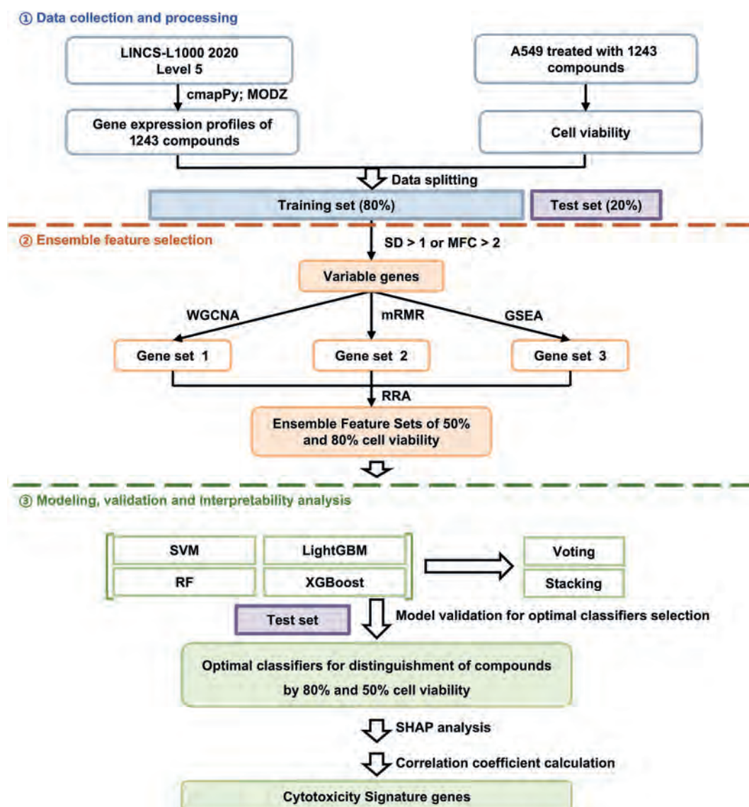
Figure 1 The schematic workflow of this study. The following models were developed for 50% and 80% cell viability prediction according to the basis of quantitative analysis of the relationship between gene signature and cell viability: (A) transcriptomic data from A549 cells treated with 1243 compounds from LINCS and cell viability data collected under the same conditions used for transcriptome data collection; (B) ensemble feature selection by using SD, MFC, WGCNA, GSEA, mRMR, and RRA algorithms; (C) and the optimal classifiers for 50% and 80% cell viability prediction were achieved by comparing various machine learning algorithms, including SVM, RF, XGBoost, LightGBM and two ensemble strategies (voting and stacking). The SHAP 35 analysis was used for interpretable analysis.
