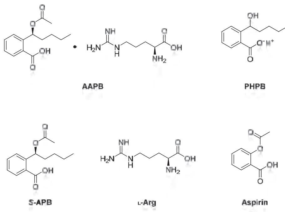
Figure 1 The structures of AAPB, PHPB, S-APB, L-Arg and Aspirin.
