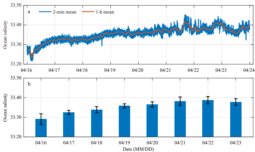
Fig. 3. The ocean salinity observed by Conductivity-Temperature-Depth Sensor at 2 m beneath the landfast ice surface during April 16–23, 2021 (a) and the daily mean salinity and standard deviation of each day (b).
