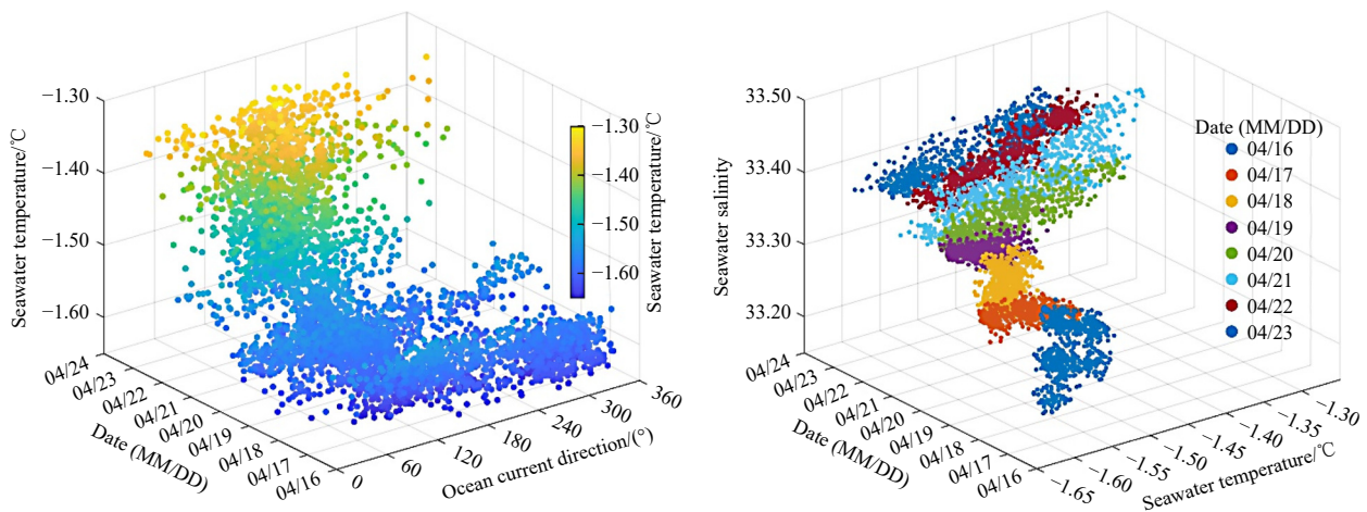
Fig. 12. The 3-D evolution of ocean current direction measured by ADV and ocean temperature measured by Conductivity-Temperature-Depth (CTD) Sensor (a) and the 3-D time-dependent distribution of ocean temperature and salinity measured by CTD (b). The observation data were obtained from April 16–23, 2021.
