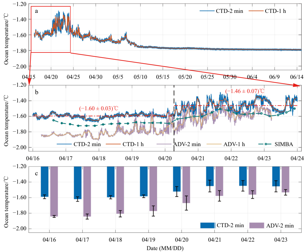
Fig. 2. The ocean temperature observed by Conductivity-Temperature-Depth (CTD) Sensor at 2 m beneath the landfast ice surface from April 16 to June 15, 2021 (a), ocean temperatures were observed by CTD, Acoustic Doppler Velocimeter (ADV) and Sea Ice Mass Balance Array (SIMBA) during April 16–23, 2021 at different locations below the landfast ice surface (b), and the mean ocean temperature and standard deviation (error bars) of each day (c). In b, the green line is the temperature obtained by the SIMBA temperature chain, the average data from five temperature sensors down the ice bottom; the blue line is the ocean temperature data measured by CTD at 2 m beneath the landfast ice surface; the purple line is the ocean temperature data measured by ADV at 5 m beneath the landfast ice surface; the horizontal coordinate of the black dotted line is the abrupt point calculated using the Mann-Kendall test (06:00 on April 20, 2021); the red dotted line is the mean ocean temperature obtained by CTD during two periods.
