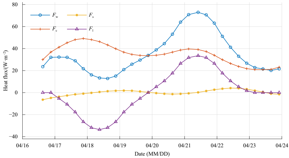
Fig. 8. Conductive heat flux ( F_c ), latent heat flux ( F_l ), specific heat flux ( F_s ) and oceanic heat flux ( F_w ) were estimated using the residual method during April 16–23, 2021. The calculation interval is 6 h.
