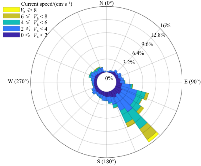
Fig. 7. Rose diagram of the 2-min mean horizontal speed ( V_h ) during April 16–23, 2021.
