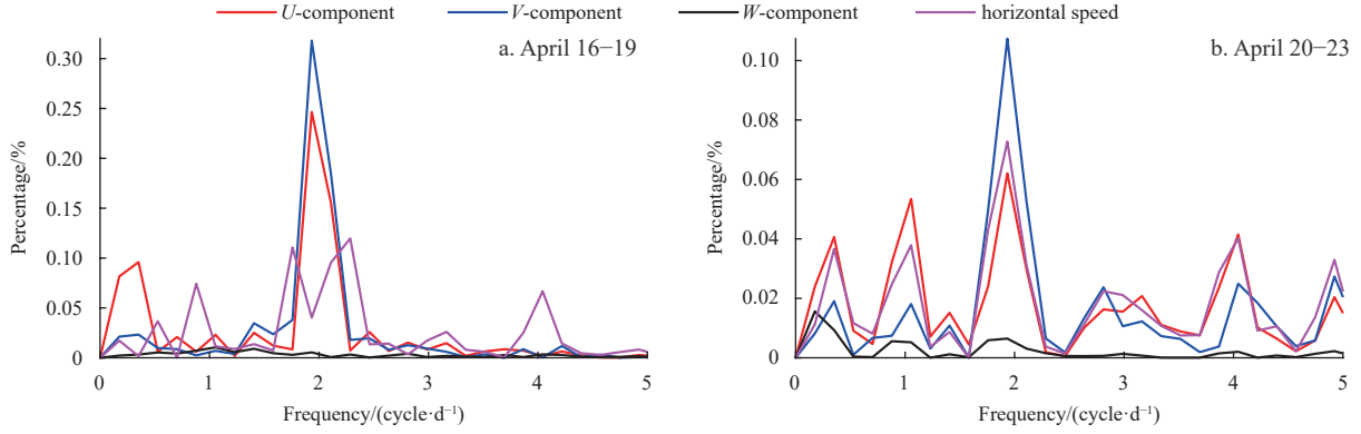
Fig. 6. The spectral analysis of ocean currents during April 16–19, 2021 (a) and April 20–23, 2021 (b), respectively. The periodogram method was used to detect the periodicity (Welch, 1967).
