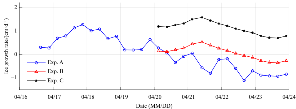
Fig. 15. Ice growth rate from different experiments of oceanic heat fluxes during April 16–23, 2021. The time interval of the calculations is 6 h.
