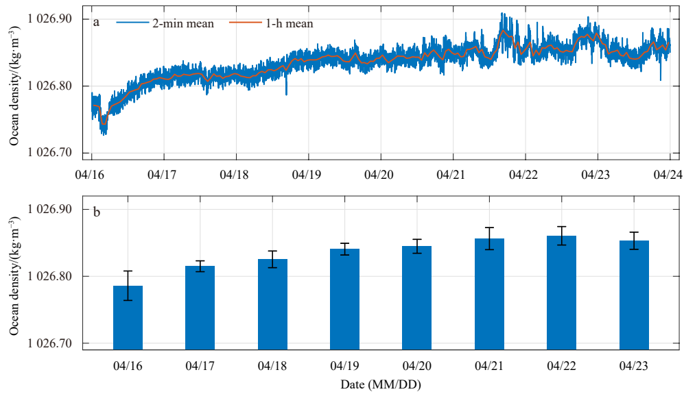
Fig. 4. The ocean density calculated by the temperature and salinity observed by Conductivity-Temperature-Depth Sensor at 2 m beneath the landfast ice surface from April 16–23, 2021 (a) and the daily mean ocean density and standard deviation of each day (b).
