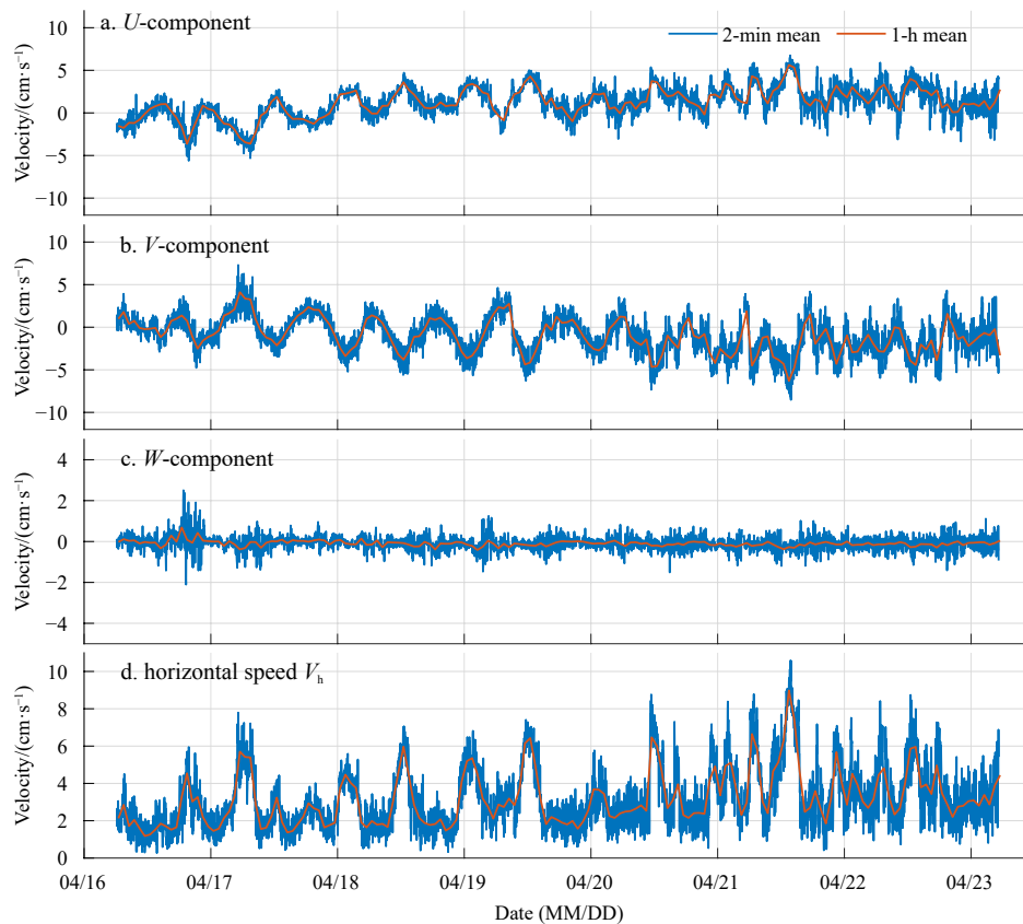
Fig. 5. The time series of ocean current velocity beneath the landfast ice observed by Acoustic Doppler Velocimeter during April 16–23, 2021. a. U -component; b. V -component; c. W -component; d. horizontal speed V_h .
