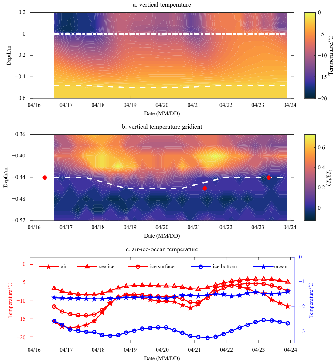
Fig. 10. Vertical temperature profiles (a), vertical temperature gradient (b), and air temperature, mean sea ice temperature (the mean of five sensors near the ice surface), ice bottom temperature (the mean of five sensors near the ice bottom), and ocean temperature (the mean of five sensors at the bottom of the temperature chain at a depth of about 3 m from the sea ice surface), recorded by Sea Ice Mass Balance Array (c). The observation data were obtained during April 16–23, 2021. In a, the white dashed line and white dash-dotted line are the ice bottom and surface, respectively. In b, the white dashed line is the ice bottom, and the red points are the ice bottom position obtained by borehole drilling.
