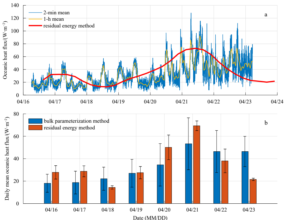
Fig. 9. High-resolution oceanic heat flux calculated by bulk parameterisation method during April 16–23, 2021 (a) and daily mean oceanic heat flux calculated by two different methods: bulk parameterisation method and residual method (b). In a, the blue and yellow lines represented 2-min mean and 1-h mean results, respectively, and the bold red lines represented oceanic heat fluxes calculated using the residual method. The error bars in b represent \pm 1 standard deviation.
