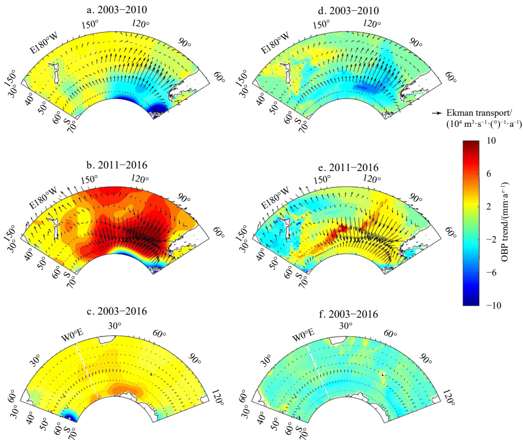
Fig. 11. Trends of OBP (color shading, mm/a) and Ekman transport (vector, \text{m}^3/(\text{°}) ) based on Grace (left panels) and PCOM (right panels). a, b, d and e. For the two periods of 2003–2010 (a, d) and 2011–2016 (b, e) in the South Pacific Ocean; c and f. for the period of 2003–2016 in the South Indo-Atlantic Ocean.
