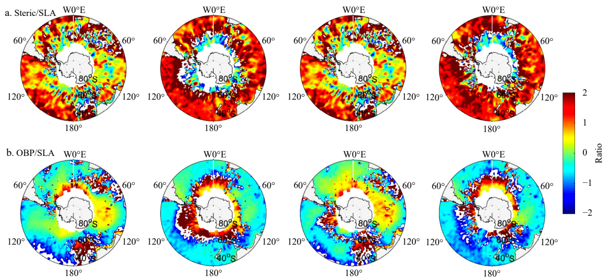
Fig. 2. Ratio of steric sea level to sea level anomaly (a), and ratio of ocean bottom pressure to sea level anomaly (b).
