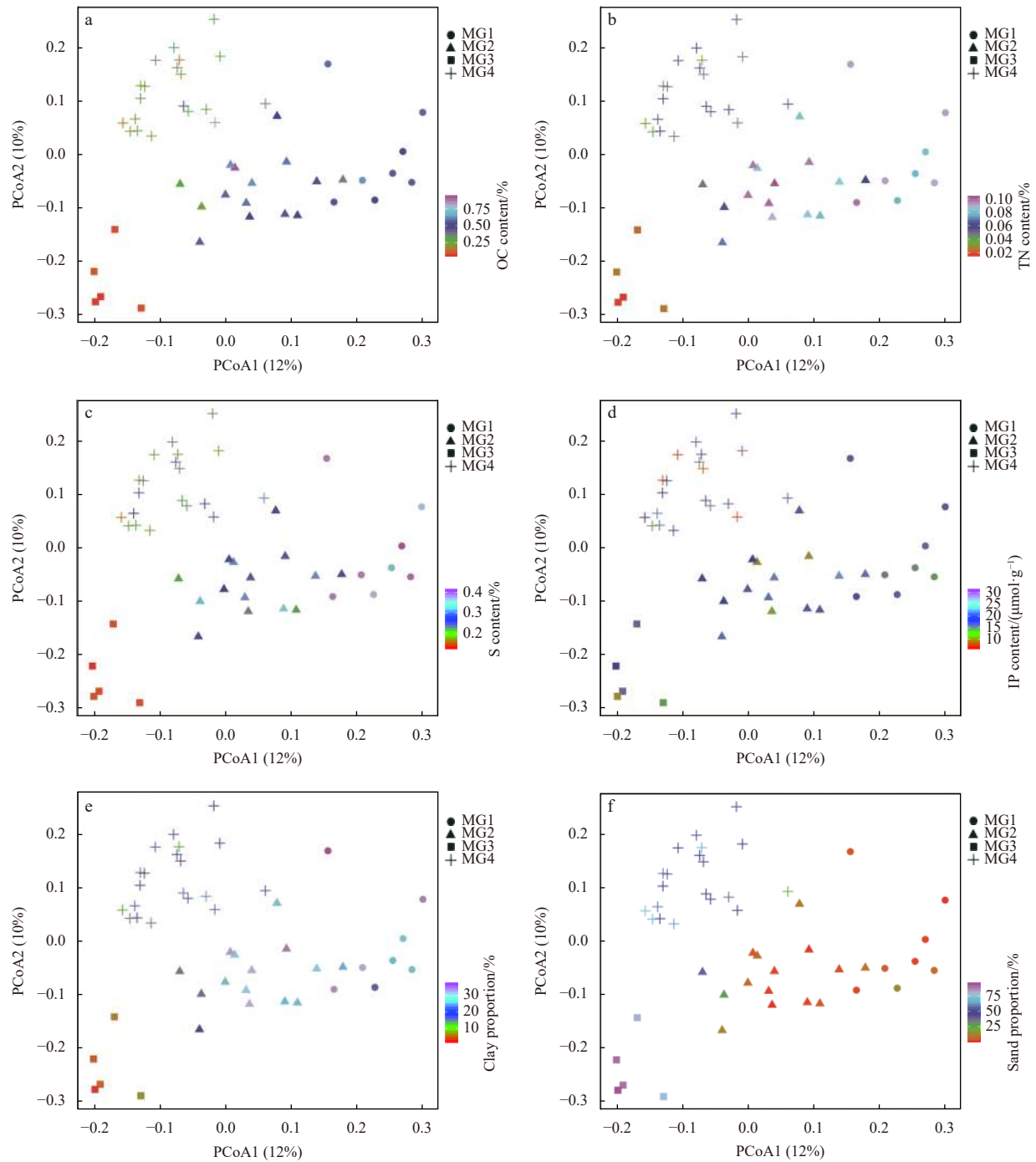
Fig. 4. Unweighted unifraco PCoA plots visualizing community dissimilarities and variations of environmental factors. OC represents organic carbon; TN, total nitrogen; S, sulfur; IP, inorganic phosphorus. The color code denotes the target environmental variable level.
