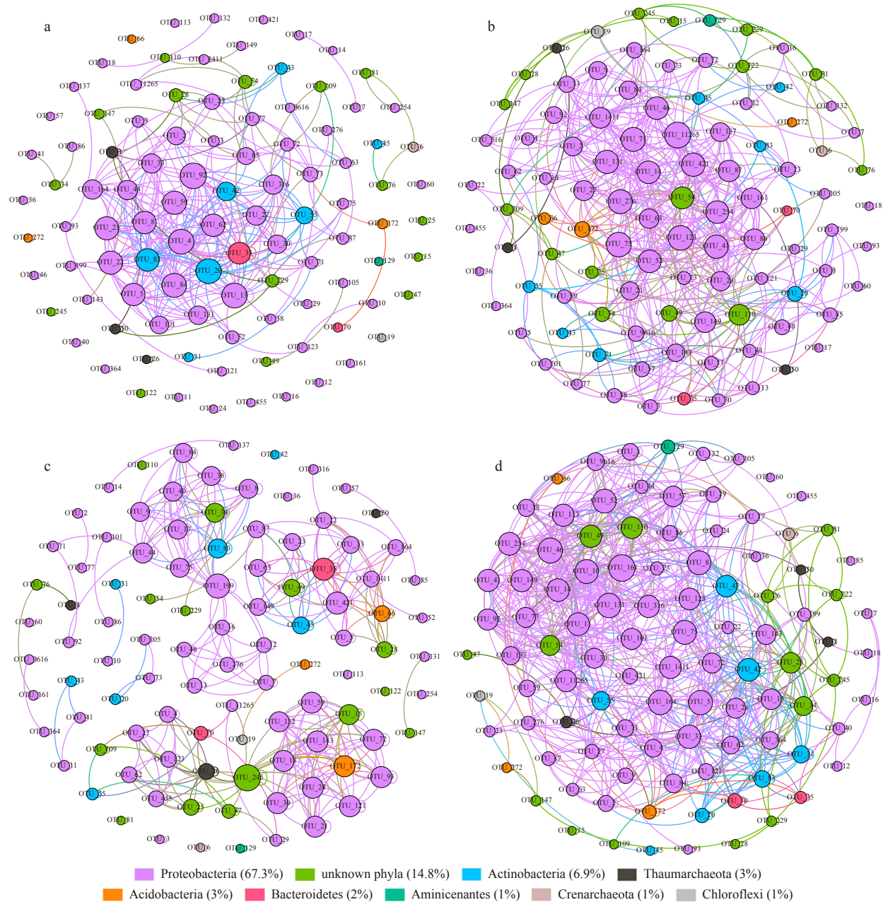
Fig. 3. Network of co-occurring OTUs in MG1 (a), MG2 (b), MG3 (c) and MG4 (d), based on correlation analysis. The selection standards for strong and significant correlation are Spearman's \rho > 0.6 and p < 0.01 , respectively. The size of each node is proportional to the relative abundance of each OTU in the network; the color and thickness of each connection between two nodes (edge) are proportional to the value of Spearman's correlation coefficients. The OTUs assigned to the same phylum were marked with the same color.
