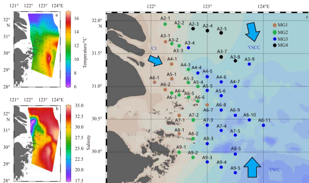
Fig. 1. Spatial distributions of temperature (a) and salinity (b) in surface waters (1 m below sea surface) in the continental shelf affected by the Changjiang River plume during March 2018 as measured with CTD vertical profiles. Dots represent CTD measurement sites. Spatial distribution of the 48 sediment samples collected in the continental shelf affected by the Changjiang River plume in March 2018 (c). The Changjiang River outflow (CJ), Taiwan Warm Current (TWC) and the Yellow Sea Coastal Current (YSCC) are schematically represented based on Kim et al. (2018).
