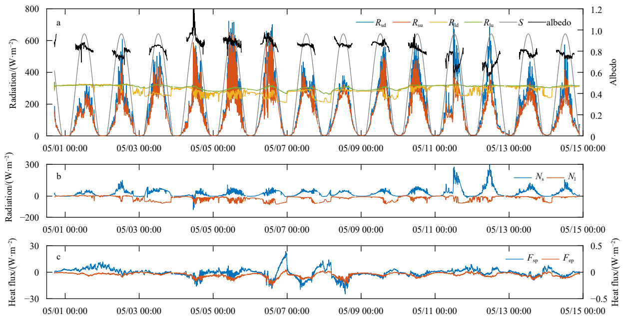
Fig. 8. Variations in radiation and heat flux on the surface of the fast ice, including the incident shortwave R_{sd} , reflected shortwave R_{su} , incident longwave R_{ld} , reflected longwave R_{lu} , solar radiation at top of the atmosphere S , and albedo (a), net shortwave and longwave radiation ( N_s and N_l ) (b), and turbulent heat flux (c). The y-axis on the right in panel c is for the latent heat flux F_{ep} .
