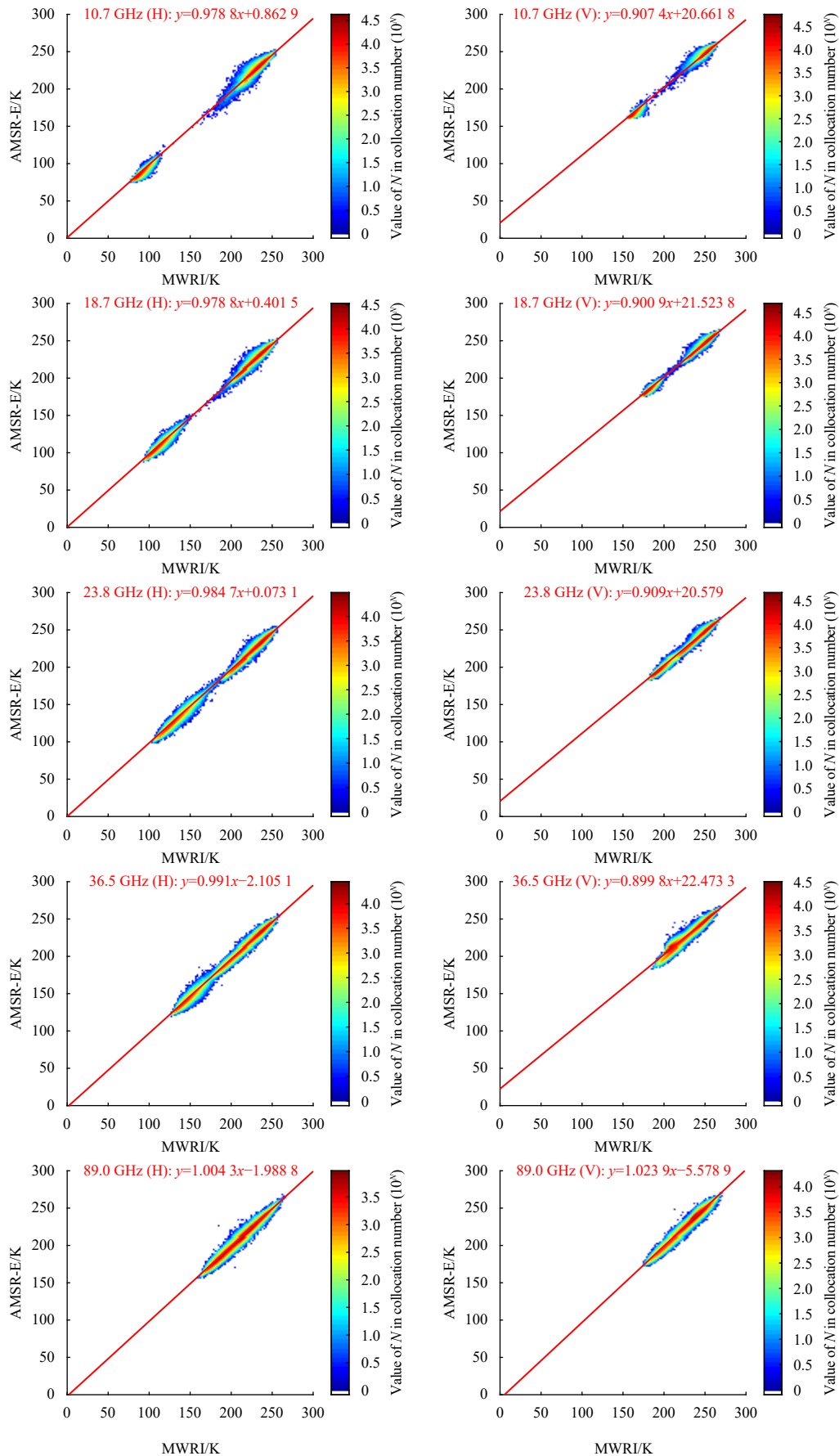
Fig. 1. Cross-calibration for 10.7–89.0 GHz (H/V polarization, ascending) in January 2011.
