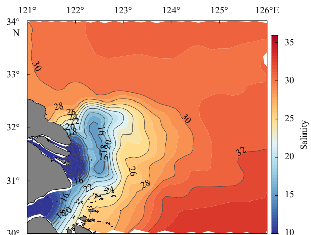
Fig. 8. Simulated surface salinity at 05:00 on August 7 in CASE06b.
