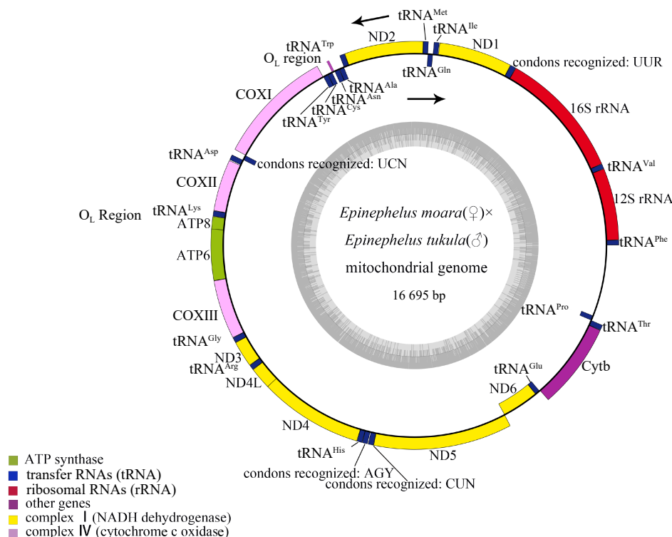
Fig. 2. Gene map of the Epinephelus moara (♀) × Epinephelus tukula (♂) mitogenome. Genes encoded on the H-strand and L-strand are shown outside and inside the circular map, respectively. ND1–ND6 represent genes of the E. moara (♀) × E. tukula (♂) dehydrogenase subunits 1–6; COXI–COXIII represent cytochrome c oxidase subunits I–III; ATP6 and ATP8 represent ATPase subunits 6 and 8, respectively; Cytb represents cytochrome b. The inner ring indicates the GC content.
