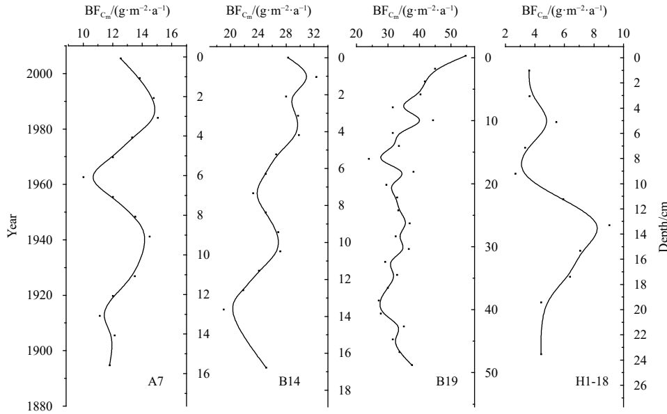
Fig. 3. The interdecadal distribution of the buried flux of marine organic carbon ( BF_{C_m} ) in cores.
