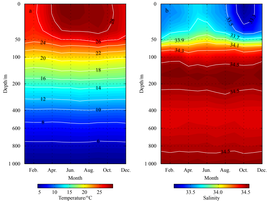
Fig. 11. Seasonal variation of mean temperature (a) and mean salinity (b) averaged in the area deeper than 1 000 m in the SCS. Contour intervals of temperature and salinity are 2^{\circ}\text{C} and 0.2, respectively.
