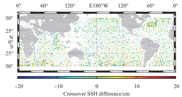
Fig. 22. Distribution of the crossover SSH differences between HY-2A and Jason-2.
