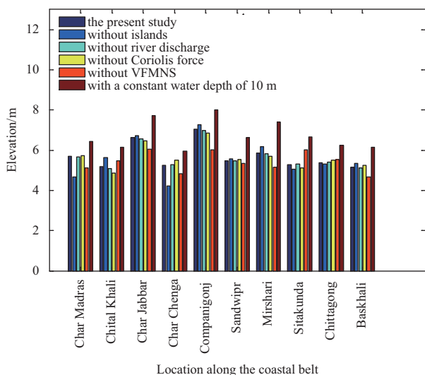
Fig. 6. Computed peak surge values by the present study and without including each of the factors, namely islands, river discharge, VFMNS, and Coriolis force keeping the other factors unchanged. Peak water levels with a constant water depth of 10 m is also presented in the figure.
