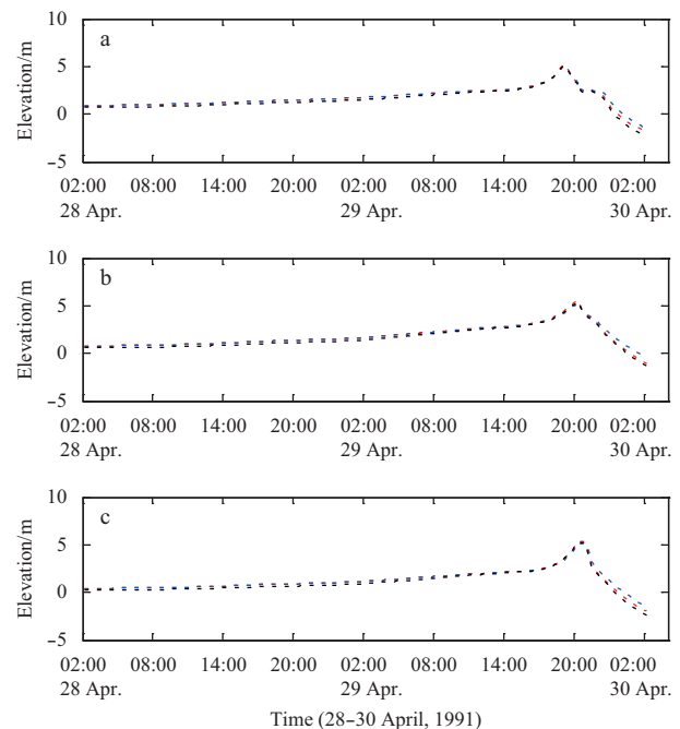
Fig. 5. Comparison of our simulated surge levels with respect to the MSL by the present study with that obtained by the MOL in coordination with the RK (4, 4) method and the FDM at Char Chenga (a), Sandwip (b) and Chittagong (c). In each case, a dotted red curve represents configuration for time variation of water levels obtained by the present study, a blue dotted curve that for the MOL in addition with RK (4, 4) method and a dotted black curve that for the FDM.
