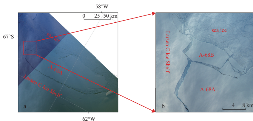
Fig. 2. GF-1 WFOV images (a) and the sub-image (b) over the new icebergs.
