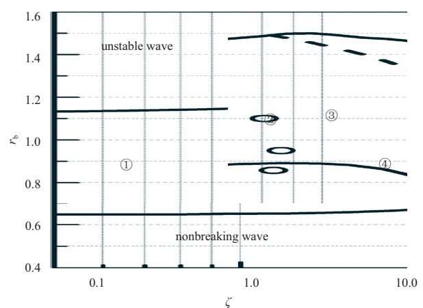
Fig. 5. Breaker type separation (Camenen and Larson, 2007).
