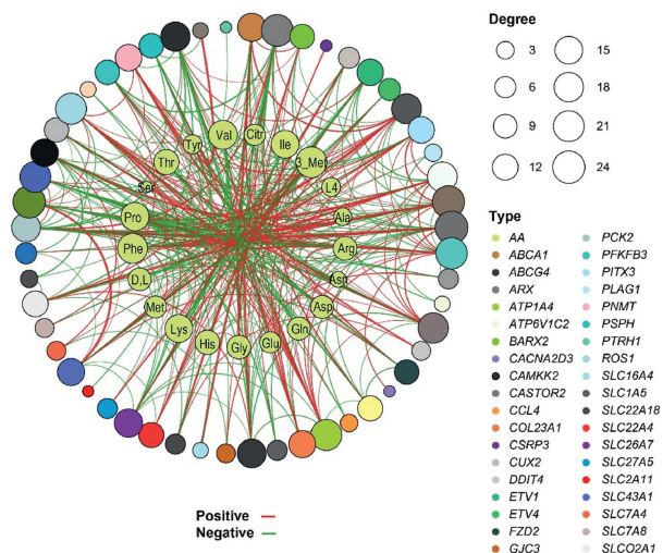
Fig. 6. The correlation network of plasma targeted metabolites of amino acids (AA) and differentially expressed genes (DEGs) in muscle tissue. The thickness of the line represents the size of correlation coefficients. The circle size represents the number of correlated relationships. Arg = arginine; Asn = asparagine; Asp = aspartic acid; Gln = glutamine; Glu = glutamic acid; Gly = glycine; His = histidine; Lys = lysine; Met = methionine; D, L = D, L-tyrosine; Phe = phenylalanine; Pro = proline; Ser = serine; Thr = threonine; Tyr = tyrosine; Val = valine; Citr = citrulline; Ile = isoleucine; 3_Met = 3-methyl-L-histidine; L4 = L-4-hydroxyproline; Ala = alanine.
