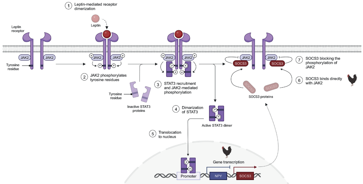
Fig. 3. Detailed leptin signaling pathway in the hypothalamus of chickens (adapted from “Cytokine Signaling through the JAK-STAT Pathway”, by BioRender.com (2023). Retrieved from https://app.biorender.com/biorender-templates ). The mechanism of leptin action in chickens may differ from what is known in mammals. In SOCS3-mediated inhibition of leptin signaling, chicken SOCS3 probably does not interact with p-Tyr986 in the intracellular domain of chicken LEPR, but directly binds to JAK2. In contrast to mammals, leptin is more likely to affect feeding behavior of chickens through the expression of the orexigenic neuropeptide NPY (but not AgRP), without affecting the expression of anorexigenic POMC. Note: The pattern of a chicken indicates differences in signaling pathway compared to mammals. LEPR = leptin receptor; JAK2 = Janus tyrosine kinase 2; STAT3 = signal transducer and transcription 3; SOCS3 = suppressor of cytokine signaling 3; NPY = neuropeptide Y.
