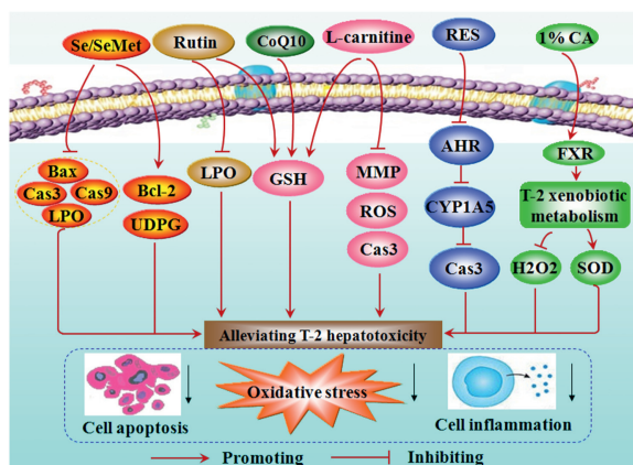
Fig. 3. The mechanisms of selenium (Se), L-carnitine, resveratrol (RES) and 1% cholic acid (1%CA) to reduce T-2-triggered hepatotoxicity. AHR = aryl hydrocarbon receptor; Bcl-2 = B-cell lymphoma 2; Bax = Bcl-2-associated X protein; Cas3 = Caspase 3; Cas9 = Caspase 9; CoQ10 = coenzyme Q10; CYP1A5 = cytochrome P450 family 1 subfamily A polypeptide 5; FXR = farnesoid X receptor; GSH = glutathione; H 2 O 2 = hydrogen peroxide; LPO = lipid peroxidation; MMP = membrane potential; ROS = reactive oxygen species; SeMet = selenomethionine; SOD = superoxide dismutase; T-2 = T-2 toxin; UDPG = UDP-glucuronosyltransferase.
