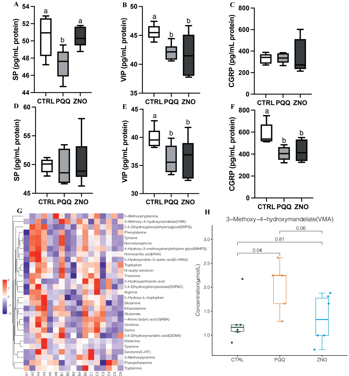
Fig. 2. Concentration of neuropeptides in plasma. (A–C) The concentration of neurotransmitters in plasma on d 14 ( n = 6 ). (D–F) The concentration of neurotransmitters in plasma on d 28 ( n = 6 ). (G) Cluster heat map of differentially expressed neurotransmitters. Red represents highly expressed neurotransmitters and blue represents lowly expressed neurotransmitters. (H) Concentration of 3-methoxy-4-hydroxymandelate (VMA) in plasma. SP = substance P; VIP = vasoactive intestinal peptide; CGRP = calcitonin gene-related peptide. CTRL, the basal diet; PQQ, basal diet supplemented with 3.0 mg/kg of pyrroloquinoline quinone disodium (PQQ·Na 2 ); ZNO, basal diet containing 1,600 mg/kg of ZnO. a,b Bars with different superscript letters are significantly different ( P \leq 0.05 ). The P -values are above the horizontal line (Fig. 2H).
