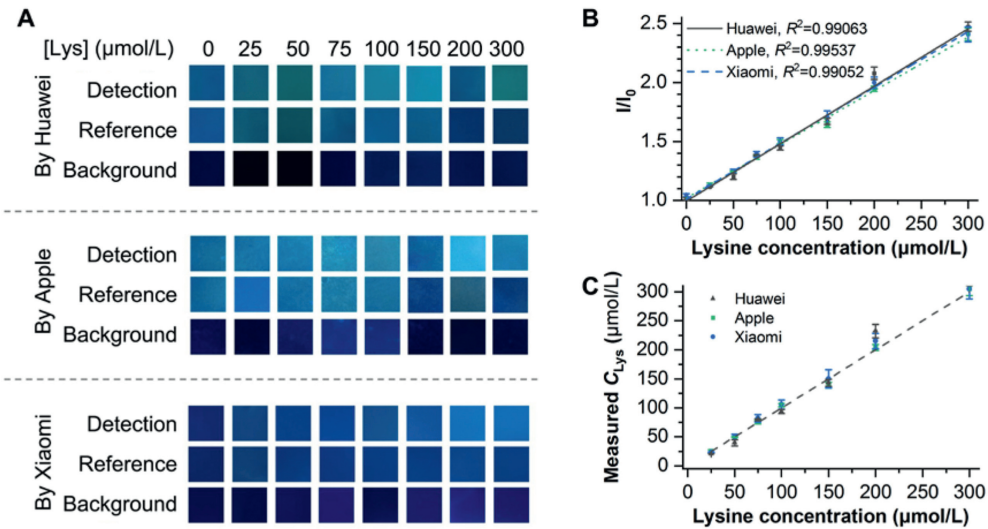
Fig. 7. The smartphone-based point-of-care testing (POCT) of lysine concentration. (A) Parts of the images captured by Huawei, Apple, and Xiaomi smartphones. (B) Linear fitting curves of the relative light intensity ( I/I_0 ) versus the concentration of lysine. (C) Concentrations of lysine measured by Huawei, Apple, and Xiaomi smartphones versus the concentration of lysine, where the calibration equation obtained by the Apple smartphone was used. C_{Lys} = the concentration of lysine.
